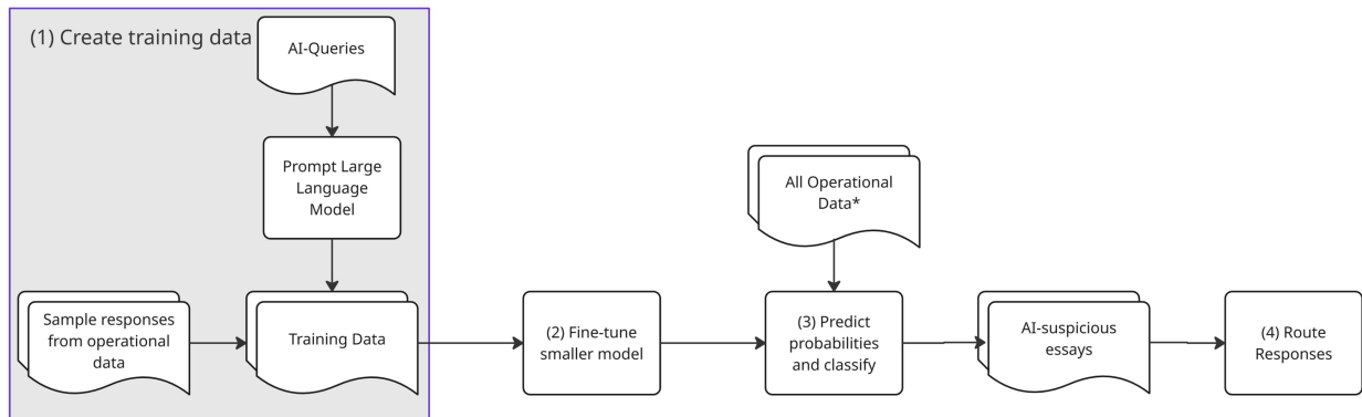
Figure 6: AI-Detection System
